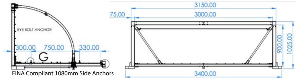
AWE394 Global Anti Goal 1.4m (above)
